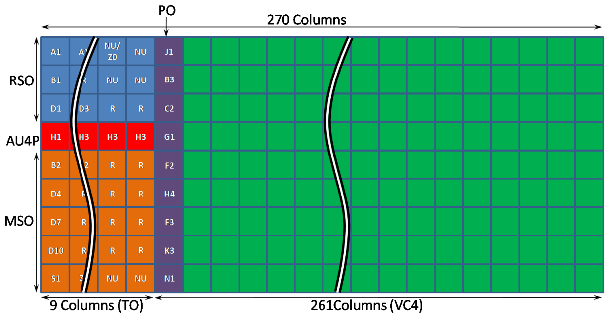
Figure 7: STM-1 frame structure
