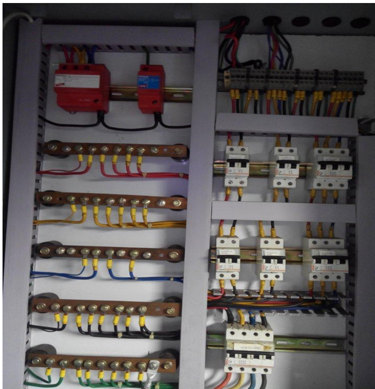
Fig18: AC Power Distribution Cabinet.
