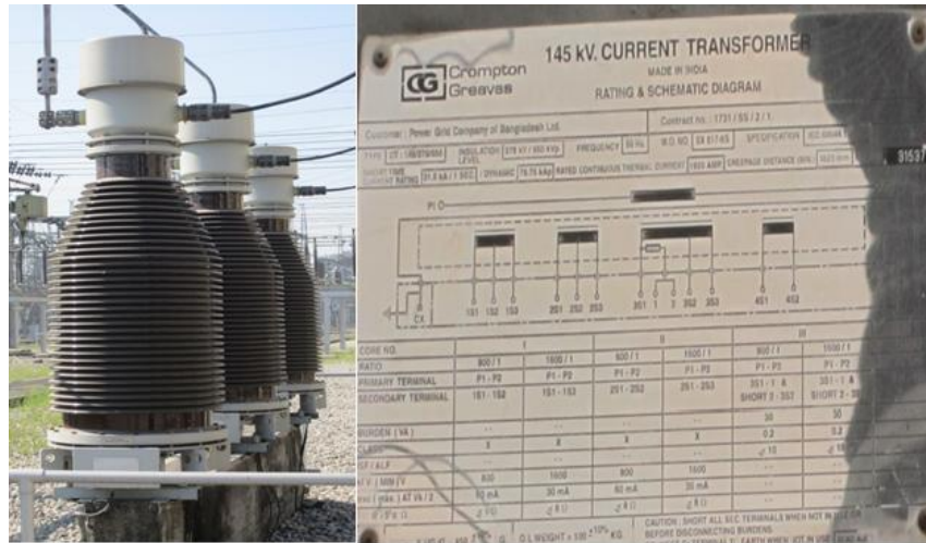
Figure 5.7: Current transformer with nameplate of the APSCL substation.
