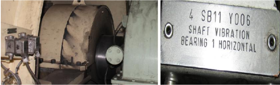
Figure 4.8: Shaft vibration sensor for unit 5 steam turbine connects with shaft.
